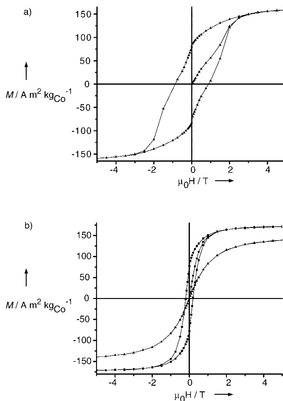
Figure 3. Plots of magnetization against applied magnetic field. a) Hysteresis loop of cobalt nanorods obtained with 1 mmol of oleylamine and 1 mmol of oleic acid: ( \blacktriangle ) measured at 300 K. b) Hysteresis loops of cobalt nanoparticles obtained with 1 mmol of oleylamine and 1 mmol of oleic acid: ( \blacksquare ) measured at 2 K, ( \blacktriangle ) measured at 300 K.
